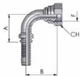
BSP FITTINGS 60° INSERTI BSP 60°
