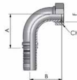
BSP FITTINGS 60° INSERTI BSP 60°
