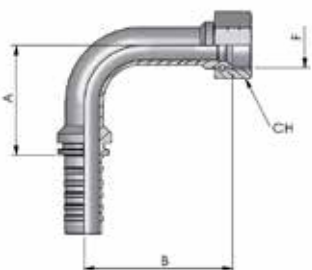
DRY-SPIRAL JIC FITTINGS 37° INSERTI JIC 37° DRY-SPIRAL
